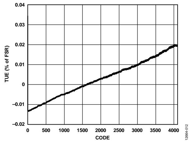
Figure 11. AD5671R TUE vs. Code
